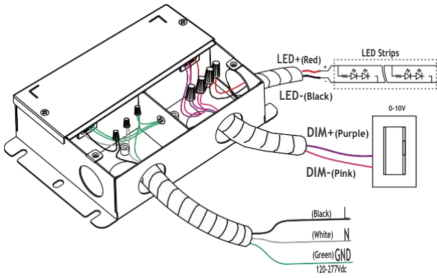
Step 5 0-10V wiring diagram
